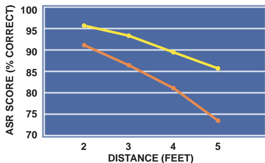
ASR SCORE VS. DISTANCE (ON AXIS, BABBLE NOISE LEVEL = 60 dB)
