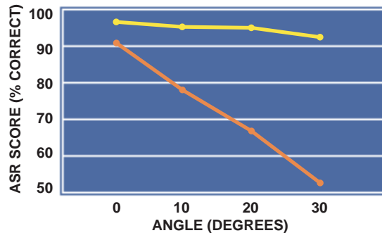
ASR SCORE VS. ANGLE (RANGE = 2 FEET, BABBLE NOISE LEVEL = 60 dB)
